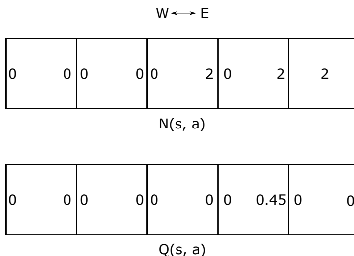
Figure 2: The N(s, a) and Q(s, a) values for the second trial/episode t_2
